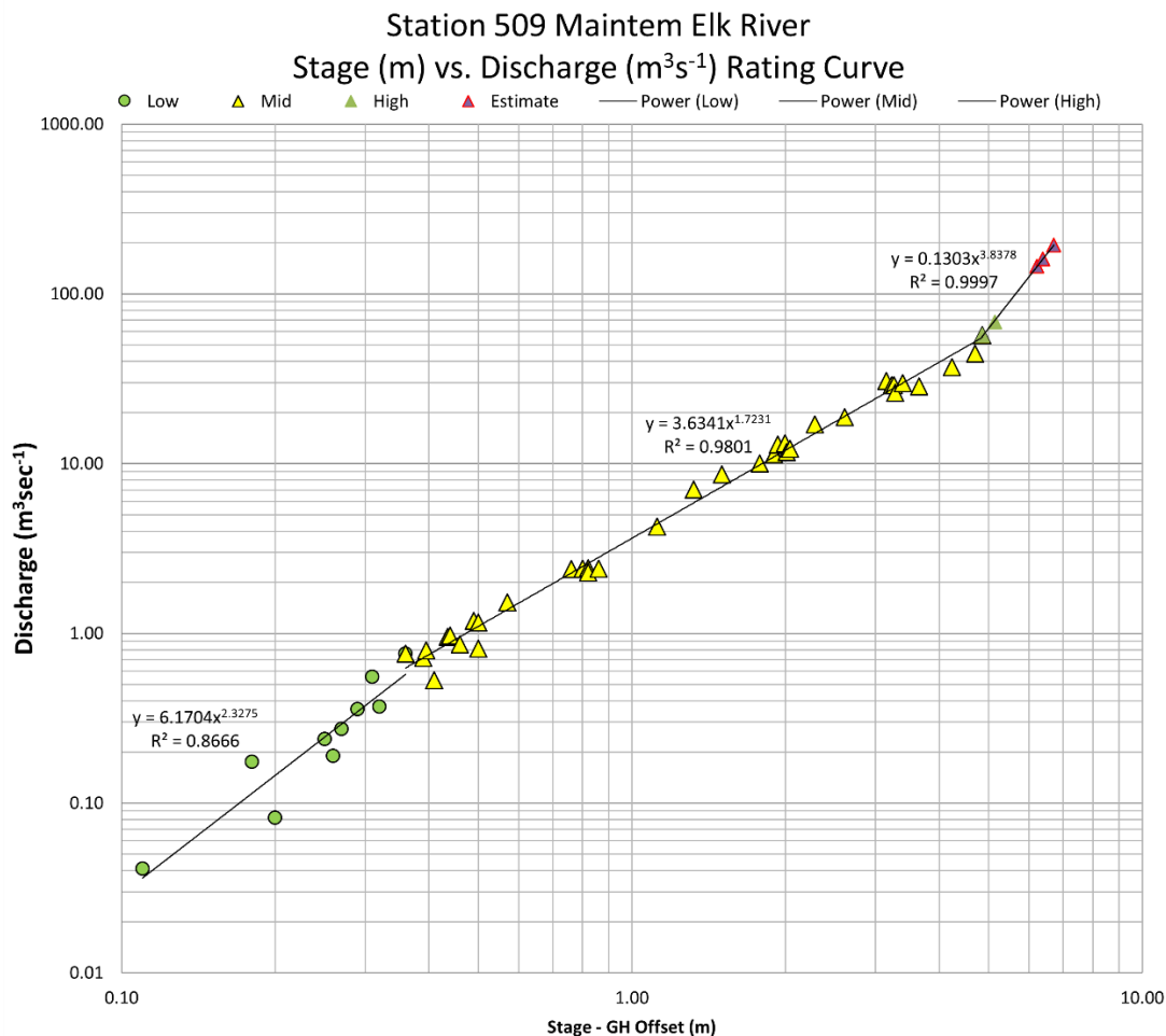
Figure 1. Stage-discharge relationship for the Mainstem Elk River gaging station 509. The gage height offset for zero flow is 0.09 meters (m).
