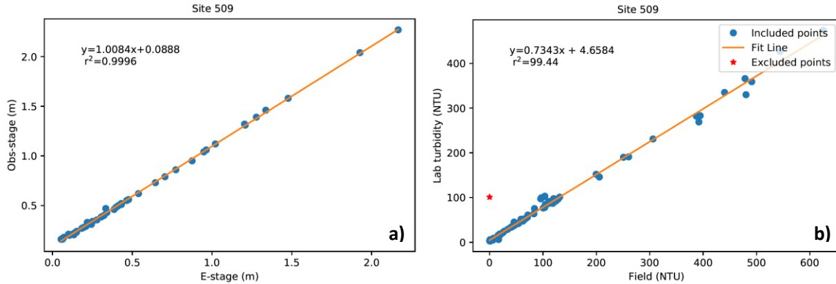
Figure 2. Instrument stage (“E-stage”) vs. observer stage (“Obs-stage”) for the Mainstem Elk River (a). Field turbidity (NTU) vs. laboratory turbidity (NTU) for the Mainstem Elk River (b).
