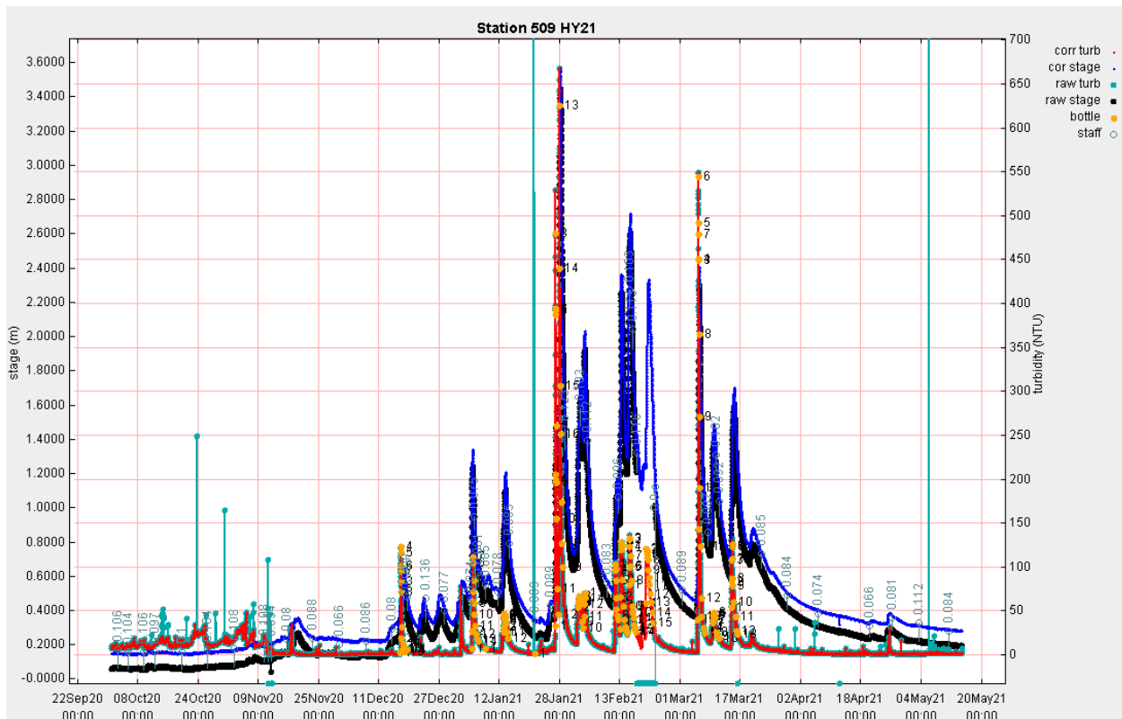
Figure 3. Corrected hydrologic data measured at Mainstem Elk River station 509, HY 2021.
